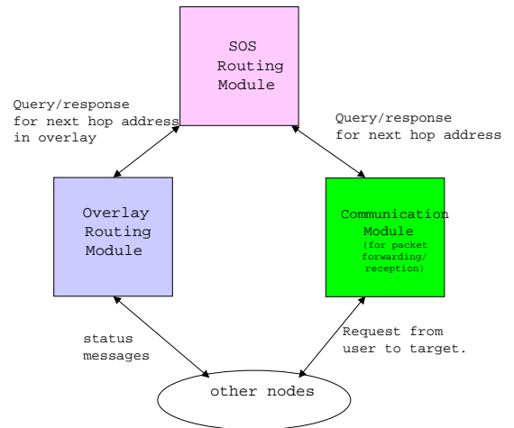
Figure 6: Software modules for the WebSOS implementation.
